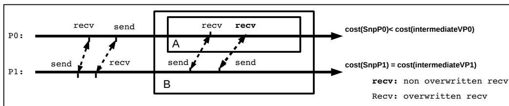
Figure 10. Representative code in which we selected two checkpointed parts
