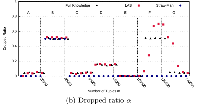
Figure 6: Simulator time-series.
