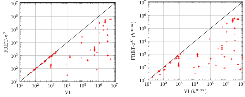
Figure 8: Cyclic planning. Number of states visited, for VI ( x ) vs. FRET- \pi^U using LRTDP _{|U} ( y ), with no pruning (left) respectively h^{\max} pruning (right).
