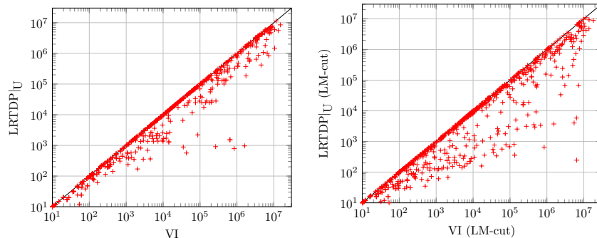
Figure 4: Acyclic planning. Number of states visited, for VI ( x ) vs. LRTDP |U ( y ), with no pruning (left) respectively LM-cut pruning (right). Default node selection.
