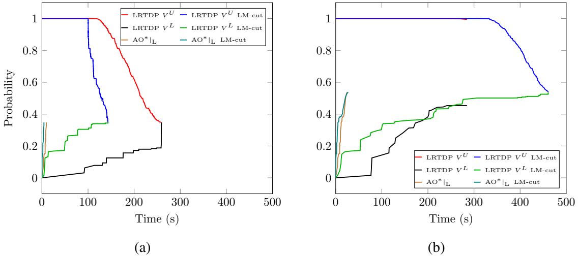
Figure 7: Acyclic planning. Anytime behavior in \text{LRTDP}|_{\text{LU}} ( V^U and V^L ) and \text{AO}^*|_{\text{L}} ( V^L only), as a function of runtime. Elevators instance 11, without pruning and with LM-cut pruning, for constrainedness level C = 1.4 (a) respectively C = 1.8 (b). Default node selection.
