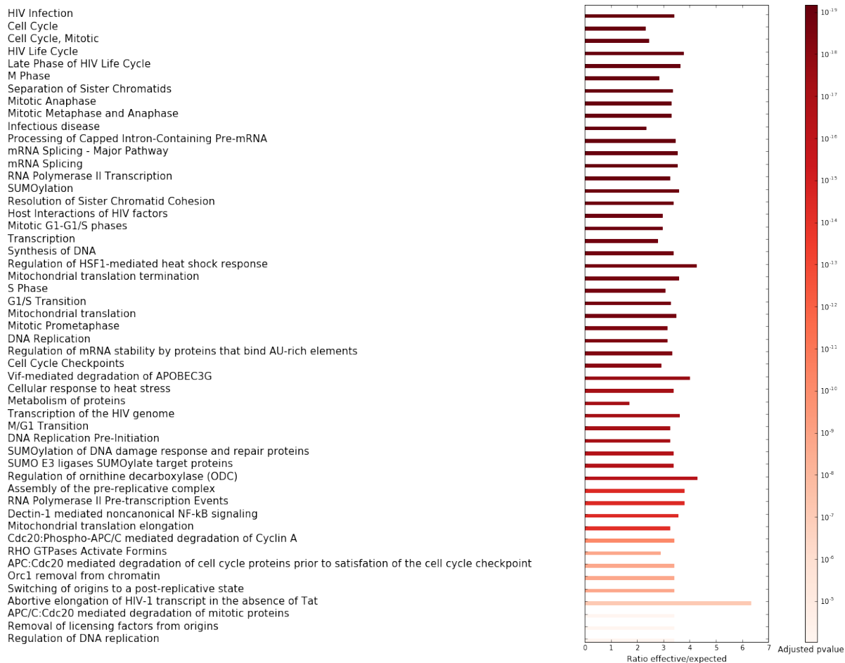
Figure 28: Significant pathway categories (at p\text{-value} = 0.001 ) of cluster 0.
