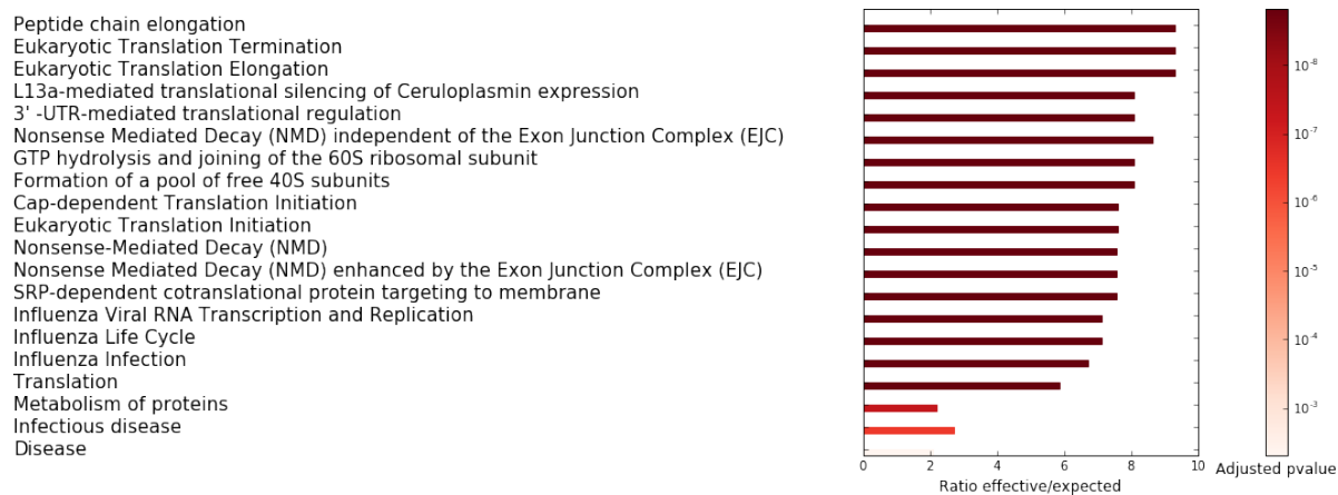
Figure 29: Significant pathway categories (at p\text{-value} = 0.01 ) of cluster 1.
