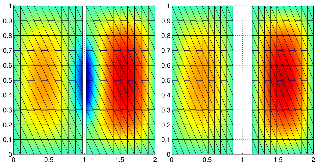
(b) Stabilized \delta -order 2 model for \delta = 0.1 .
