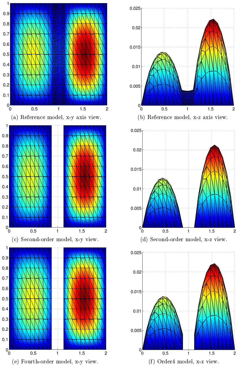
Figure 5: Solution to the reference Problem (2), the second-order model (22) and the fourth-order model (23) of the first class.
