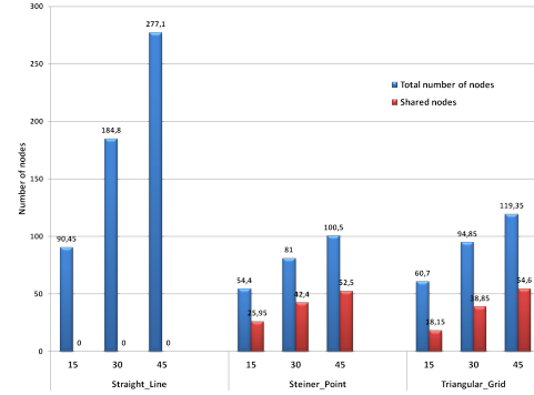
Fig. 6: Total and shared nodes deployed.
