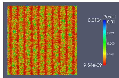
Figure 5.7: Absolute error between the exact solution and the solution computed with the HDG- \mathbb{P}_2 scheme on mesh M1.
