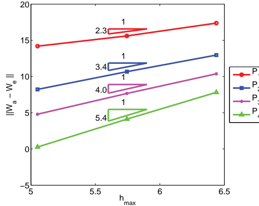
Figure 5.10: Convergence order of HDG method for plane wave propagation in a homogeneous medium.
