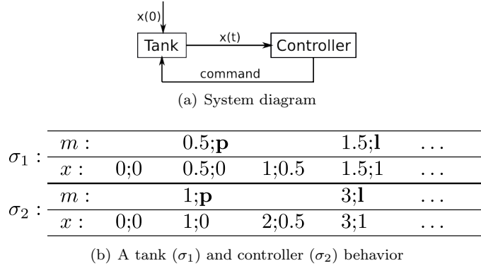
Figure 1: Water controlling system
