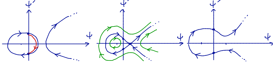
FIGURE 1. Portraits of the curve y^2 = f(x) parameterized by (\Psi, \Psi') . From left to right: case (i) H \in (c(A, q), h(A, q)) (the red part corresponds to t \in [0, 1] ), (ii) H = h(A, q) (phase portrait in green for other boundary conditions close to the saddle equilibrium), (iii) H > h(A, q) .
