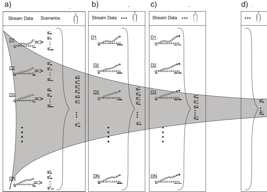
Fig. 7. Method of application of the relational database data for the analysis of streaming data.
