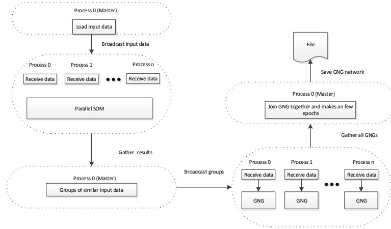
Fig. 2. Parallel Algorithm
