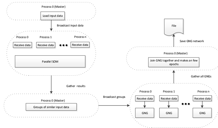
Fig. 2. Parallel Algorithm
