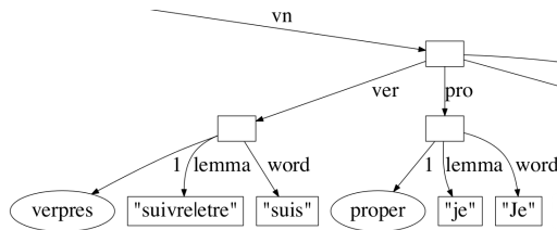
Fig. 5. Excerpt of the composition modelling for the phrase "Je suis".
