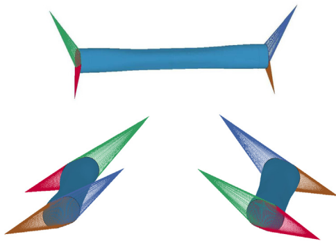
Fig. 6. The initial shape of the twist beam used—visualization from different sides by the software Ls Dyna.
