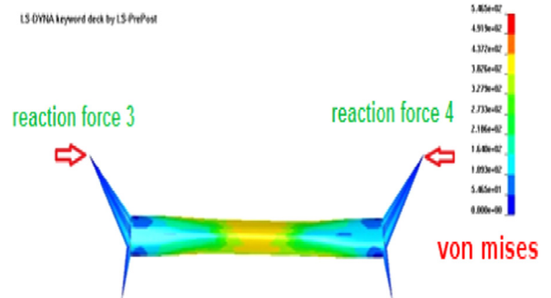
Fig. 7. Two criteria to be optimized “ FR_{34} vs VM ”: the first criterion and the second one present the rigidity and the resistance to fatigue, respectively.
