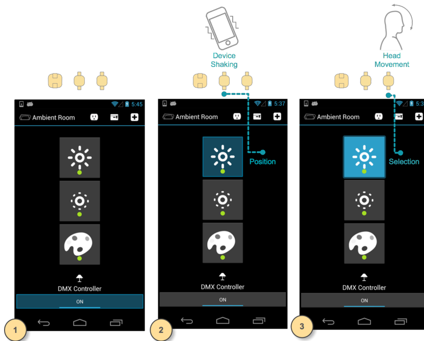
Fig. 7. AmbientRoom application NUI-enabled Interactions
