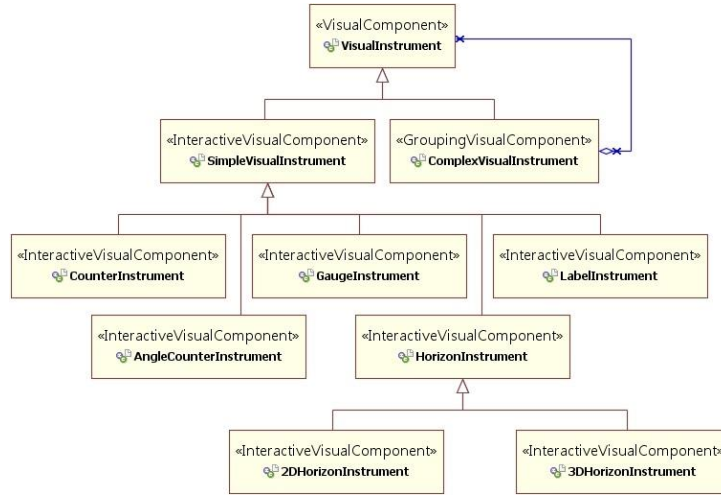
Figure 13. Hierarchy of common visual instrument types described in terms of the UML Stereotypes.
