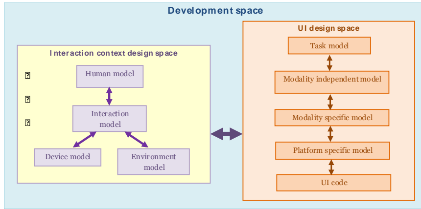
Figure 5. Combining UI and interaction design spaces.
