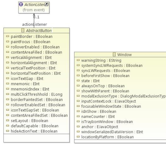
Figure 9. Java GUI controls as UML classes.
