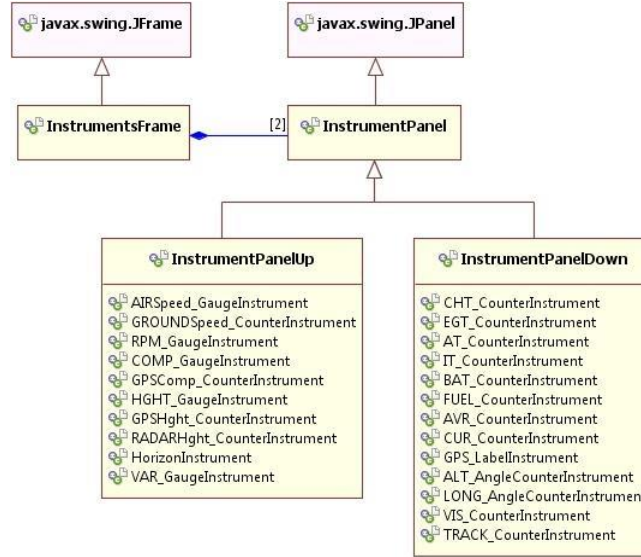
Figure 15. Platform-specific software instrument table model.
