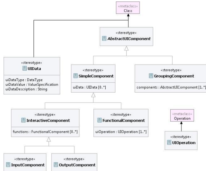
Figure 7. Basic UML Stereotypes for AUI design.
