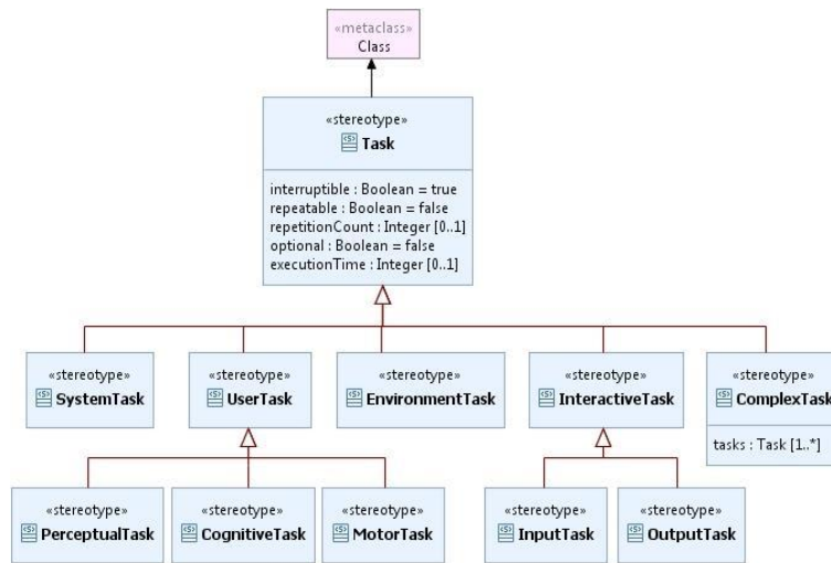
Figure 6. Basic UML Stereotypes for task design.
