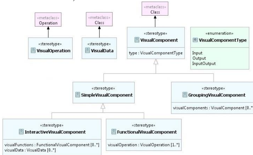
Figure 8. Basic UML Stereotypes for visual UI design.
