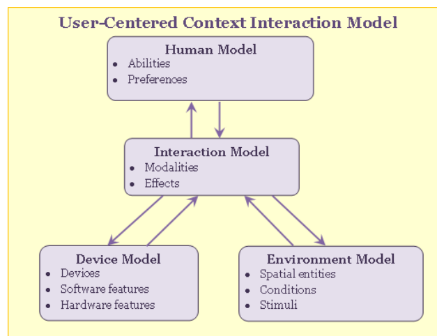
Figure 1. High-level view on unified user-centered interaction model.
