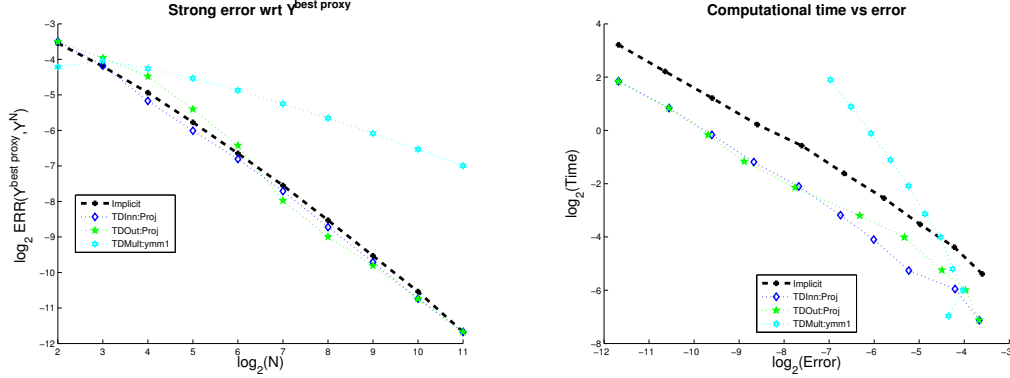
Figure 6.1: Errors computed for N \in \{4, 8, 16, \dots, 2048\} , with M = 100k and K = 10 .
