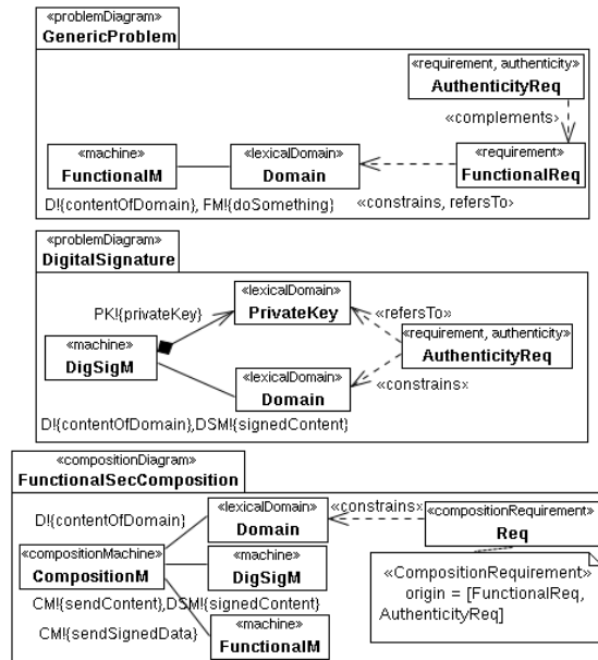
Fig. 1. Problem-oriented digital signature pattern (graphical pattern)
