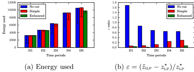
Figure 2: Comparison of the performance of different Column Generation Models for pdh .
