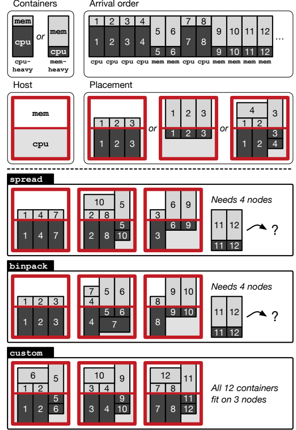
Figure 1. Placement of the containers with 3 scheduling strategies for a given arrival order of containers, and assuming that a node can host 3 cpu-heavy containers, or 3 mem-heavy containers, or 2 of each type (top). While spread and binpack would require 4 nodes to schedule 12 containers, custom requires only 3 (bottom).
