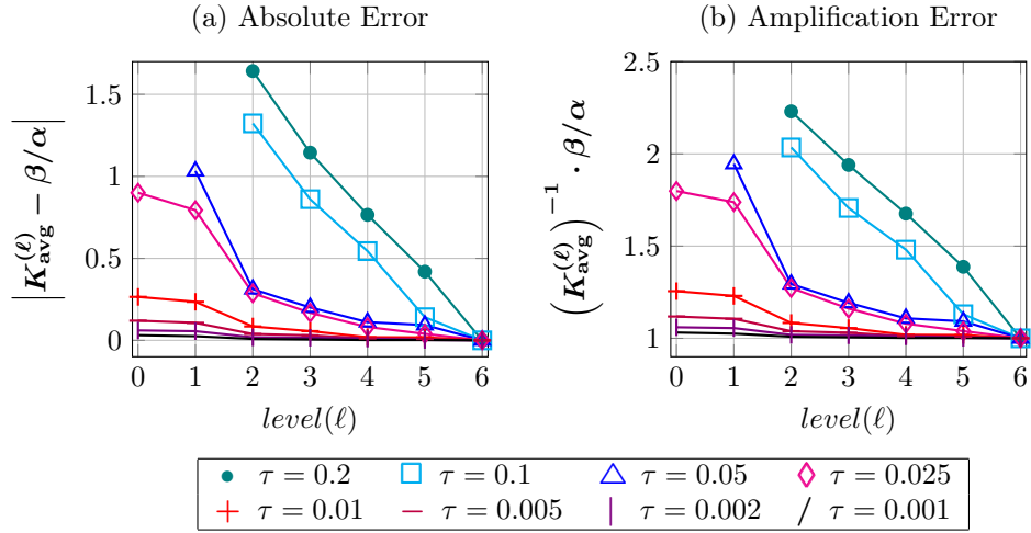
Figure 12: Avg. Condition Number Error vs. Level.
