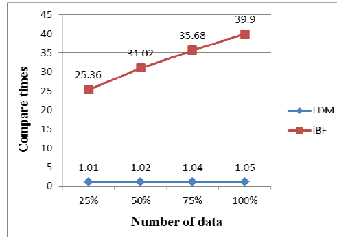
Fig. 3. The average comparison times in Data Duplication
