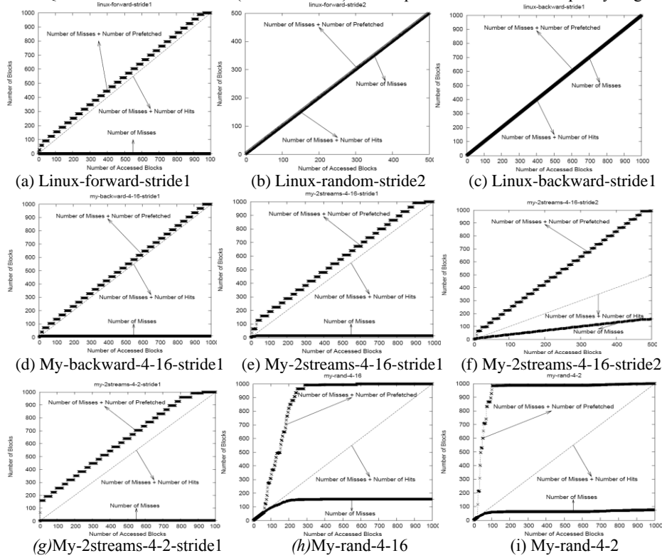
Figure 1. The various curves of performance characteristics of the two prefetching policies
