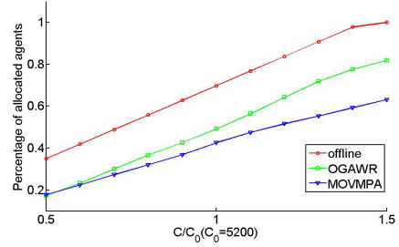
Fig. 5. The sum of agents value under three mechanisms
