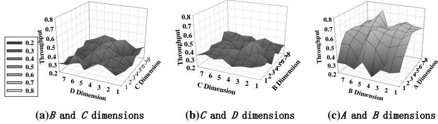
Fig.10. Load balancing condition of 4.5D torus network
