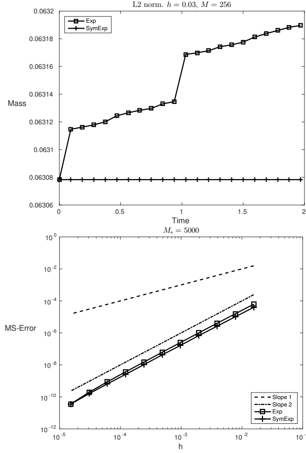
Figure 5.1: Preservation of the L^2 -norm (top) and mean-square errors (bottom) for the symmetric exponential integrator (5.1) (+) and for the exponential integrator (3.1) ( \square ). The dotted lines have slopes 1 and 2.
