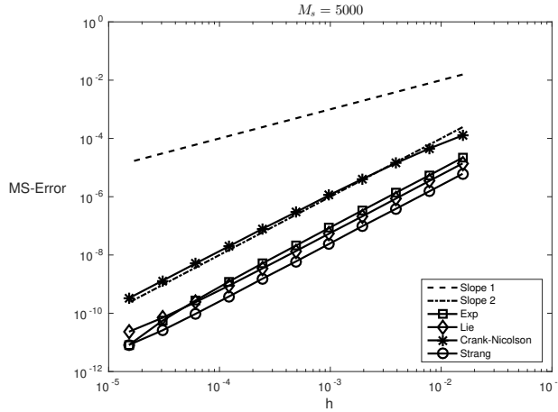
Figure 4.2: Mean-square errors for c = 0.25 : Exponential integrator ( \square ), Lie-Trotter ( \diamond ), Crank-Nicolson ( * ), Strang ( \circ ). The dotted lines have slopes 1 and 2.
