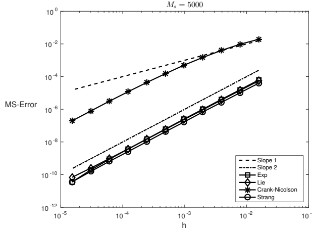
Figure 4.1: Mean-square errors for c = 1 : Exponential integrator ( \square ), Lie-Trotter ( \diamond ), Crank-Nicolson ( * ), Strang ( \circ ). The dotted lines have slopes 1 and 2.
