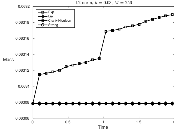
Figure 4.5: Preservation of the L^2 -norm: Exponential integrator ( \square ), Lie-Trotter ( \diamond ), Crank-Nicolson (*), Strang ( \circ ).
