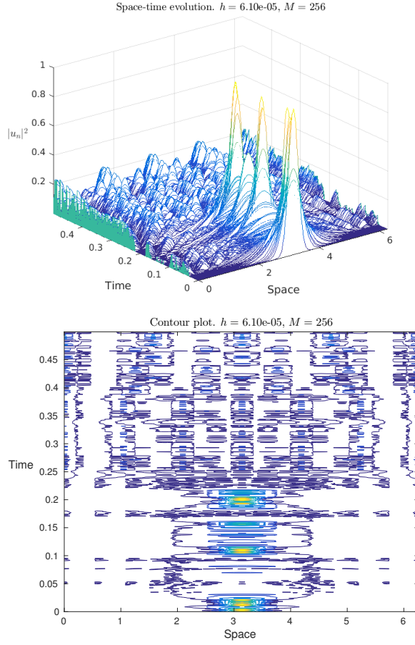
Figure 4.3: Space-time evolution (up) and contour plot (bottom) for the exponential integrator (3.3).
