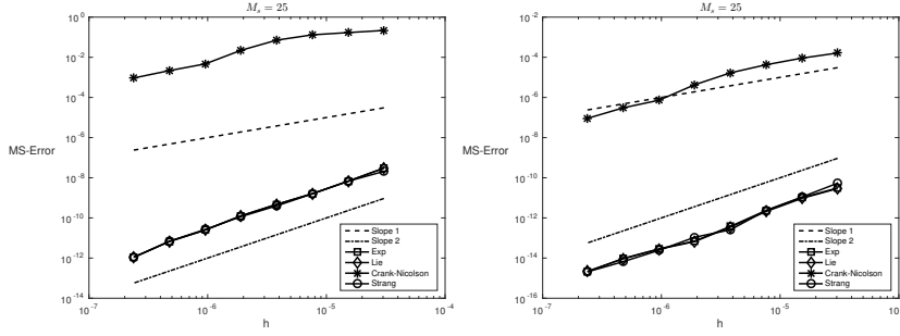
Figure 4.6: Mean-square errors in 2d for c = 1 (left) and c = 0.1 (right): Exponential integrator ( \square ), Lie-Trotter ( \diamond ), Crank-Nicolson (*), Strang ( \circ ). The dotted lines have slopes 1 and 2.
