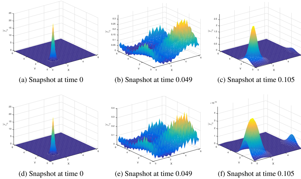
Figure 4.7: Snapshots of the evolution of the exponential integrator in 2d : \sigma = 1.9 (up) and \sigma = 2 (bottom). Discretisation parameters: h = 2^{-11} and M = 2^7 . Note the scale on the z -axis on Figure 4.7f.
