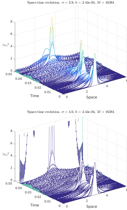
Figure 4.4: Space-time evolution for the exponential integrator: \sigma = 3.9 (up) and \sigma = 4 (bottom).
