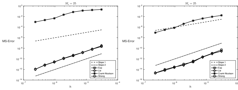
Figure 4.6: Mean-square errors in 2d for c = 1 (left) and c = 0.1 (right): Exponential integrator ( \square ), Lie-Trotter ( \diamond ), Crank-Nicolson ( * ), Strang ( \circ ). The dotted lines have slopes 1 and 2.
