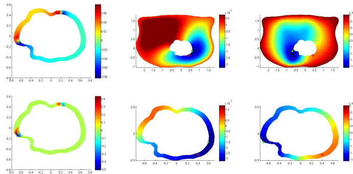
Figure 3 – Top (left) : the solution u_e at 20 ms, Bottom (left) : the source. Top (Middle) (respectively, Top (right)) The topological gradient for the cost function \mathfrak{J}_1 (respectively, \mathfrak{J}_2 ) in the heart thorax doamin. Bottom (Middle)(respectively, Bottom (right)) : The topological gradient for the cost function \mathfrak{J}_1 (respectively, \mathfrak{J}_2 ) in the heart doamin.
