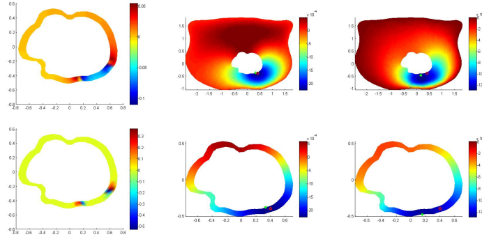
Figure 2 – Top (left) : the solution u_e at 4 ms, Bottom (left) : the source. Top (Middle) (respectively, Top (right)) The topological gradient for the cost function \mathfrak{J}_1 (respectively, \mathfrak{J}_2 ) in the heart thorax doamin. Bottom (Middle)(respectively, Bottom (right)) : The topological gradient for the cost function \mathfrak{J}_1 (respectively, \mathfrak{J}_2 ) in the heart doamin.
