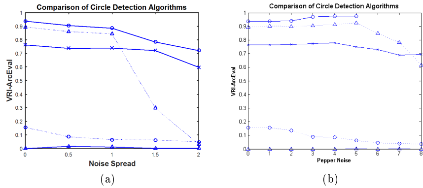
Fig. 8: The average Liu-Dori VRI across the 10 images for (a) edge and (b) pepper noise when arcs are eliminated from the ground truth. The legend is as in Figure 5.
