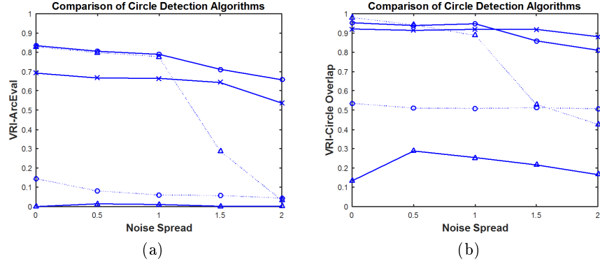
Fig. 6: The average VRI across the 10 instances and 10 images for edge noise (a) Liu-Dori metric (b) Circle overlap metric. The legend is as in Figure 5.
