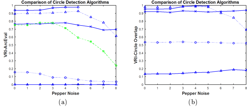
Fig. 7: The average VRI across the 5 instances and 10 images for pepper noise (a) Liu-Dori metric (b) Circle overlap metric. The legend is as in Figure 5. In Figure (a) the dashed line with square symbols is results from paper [13]
