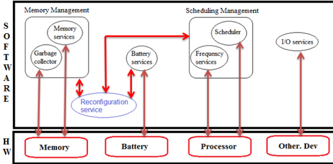
Figure 3. OS services.
