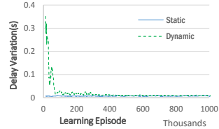
Fig. 5. Delay Variation
