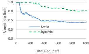
Fig. 4. Acceptance Ratio
