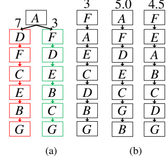
Figure 13: Ordering of paths in Figure 11. (a) the order starting from F and the green order starting from A have the smallest number of gaps (3). The red order starting from A has the largest (7). (b) When considering the concavity of the surface at the gaps, the order starting from A has a score of 5.0 while the order starting from F has a smaller score of 4.5.
