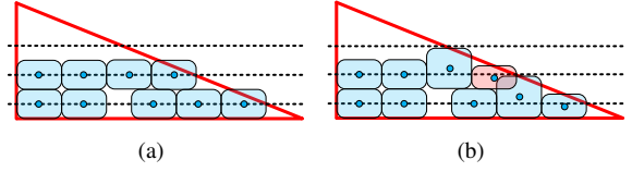
Figure 7: Raising the toolpaths may produce small overlaps where toolpaths do not align across layers. (a) Original uniform slice, viewing the cross section of the deposited plastic tracks. (b) Anti-aliased layer with displaced plastic tracks, revealing the overlap.
