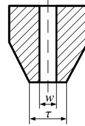
Figure 9: Typical nozzle geometry, sectional view. w is the inner diameter, \tau is the outer diameter.
