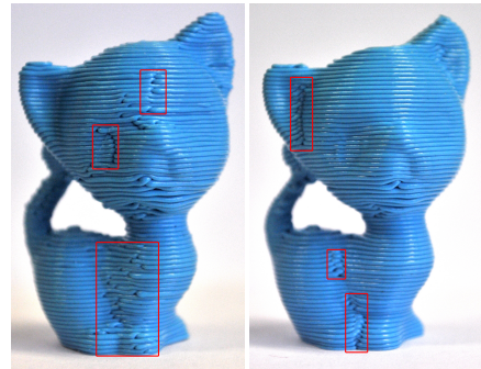
Figure 14: Hiding seams. Seams are highlighted with red rectangles. Left: No optimization of seams. Right: Result after our algorithm. Most of the visible gaps exist on the print without our technique (extrusion start/stops, also called zippers).
