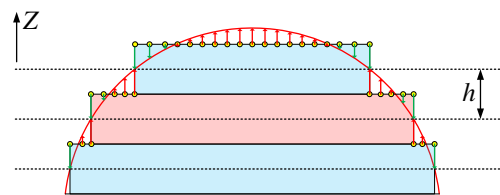
Figure 3: 2D illustration of uniform slicing (side view). The red curve is the input model boundary. The blue and red rectangles are cut view of the layers. Dashed lines are the mid-layer slicing planes. The layers are vertical extrusions of the intersection between the slicing planes and the initial object. The yellow circles are points on the top of the layers, that form the physical object boundary. The arrows reveal the distance between the printed surface and the true surface (red: positive; green: negative).
