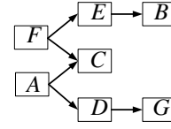
Figure 12: Height constraint graph for the example in Figure 11
