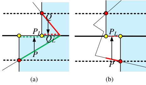
Figure 5: (a) Displacing both the bottom and top of layers correctly opens a tear between two adjacent layers. (b) Surfaces folding more than once within the slice cannot be properly approximated.
