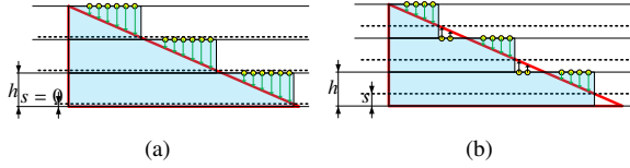
Figure 8: Left: s = 0 produces only downwards displacements, but exceeds the lower thickness bound. Right: Intermediate values less than \frac{h}{2} exploit thinner slices while reducing overlaps across layers.
