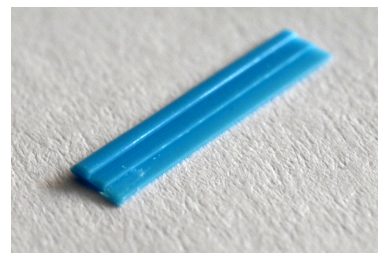
Figure 10: Interference between neighboring paths. (a) The heights of A, B and C are: 0.1mm, 0.3mm and 0.6mm. The distances between the middle axis of A, B and C are w = 0.8 mm, which is smaller than the nozzle outer diameter \tau = 1.25 mm. (b) Printed result in the order C, B, A . (c) Printed result in the order A, B, C
