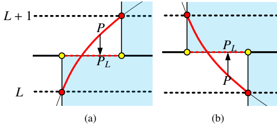
Figure 4: Illustration of the mapping between surface points and layers for the case of respectively top-facing (a) and bottom-facing (b) surfaces. The dashed black lines are mid-layer slicing planes. The dashed red segment is a physical boundary of the printed shape, at the top (a) or bottom (b). Each surface point P vertically projects to a point P_L on this segment. If the mapping is injective we can snap the points P_L back to the surface. The displacement is \pm \frac{h}{2} at most.
