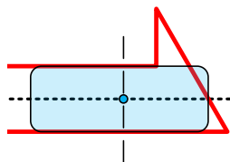
Figure 20: The blue rectangle is a cross-section of a printed plastic path. The red outline is the shape of the anti-aliased layer. The only degree of freedom to deform the path is the blue vertex. In such a case, the toolpaths cannot be modified to reproduce the sharp features of the anti-aliased layers.
