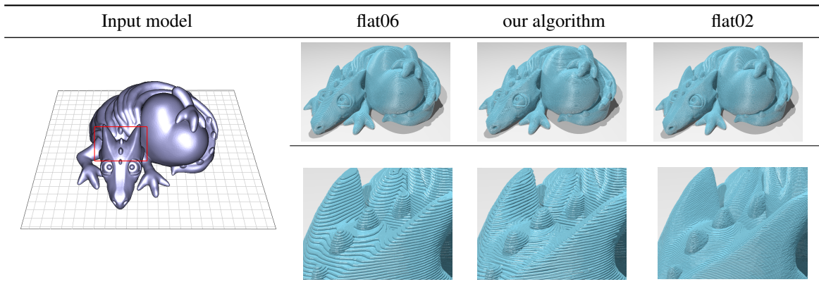
Figure 17: Rendered printouts of "Pet monster Valentine" (thing: 17204). Leftmost column: input 3D model and closeup regions outlined with red rectangle. Second column: flat06, general and closeup views. Third column: our result, general and closeup views. Fourth column: flat02, general and closeup views.
