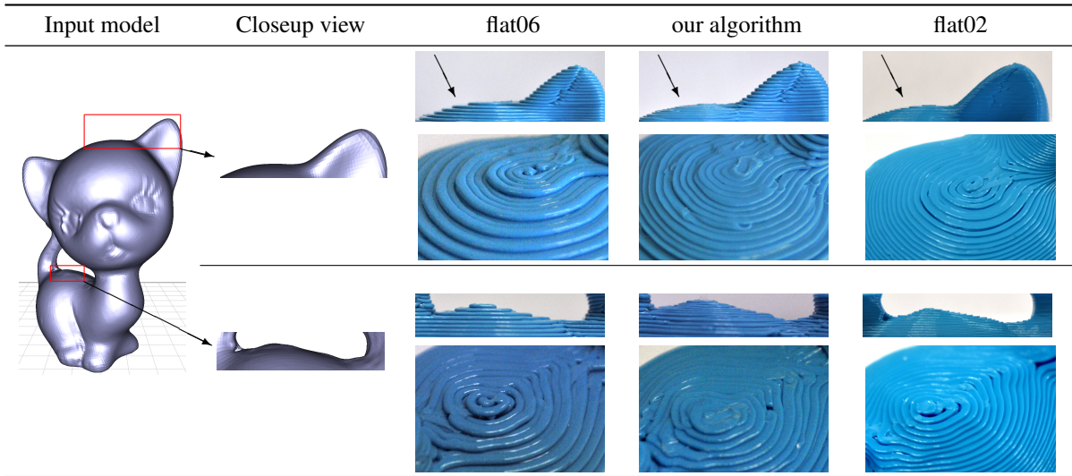
Figure 15: Real printouts of "Kitten" (thing: 12694). Leftmost column: input 3D model and closeup regions outlined with red rectangles. Second column: 3D model, closeup views. Third column: flat06, side and top views on real printout. Fourth column: our result, side and top views. Fifth column: flat02, side and top views.
