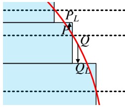
Figure 6: Mapping between surface points P and Q and layer tops/bottoms in adaptive slicing (respectively P_L and Q_L ). The magnitude of the displacements remains bounded by half the layer thickness, but the actual value depends on which layer top/bottom is displaced.
