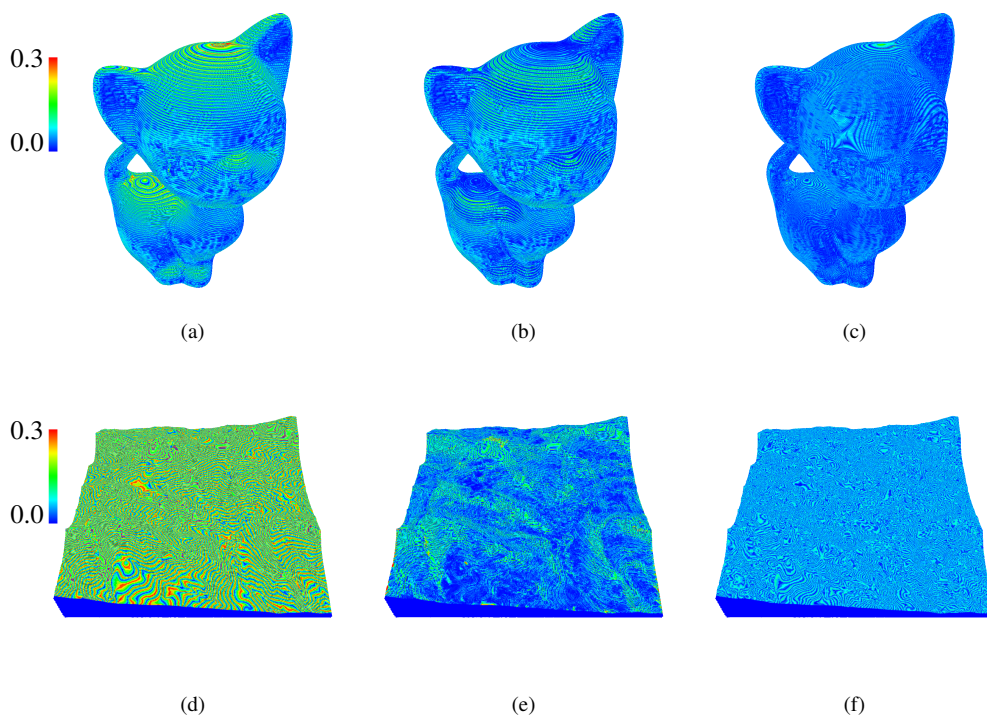
Figure 19: Error map of "Kitten": (a) flat06, (b) our algorithm, (c) flat02, and "Lassen Volcanic": (d) flat06, (e) our algorithm, (f) flat02.
