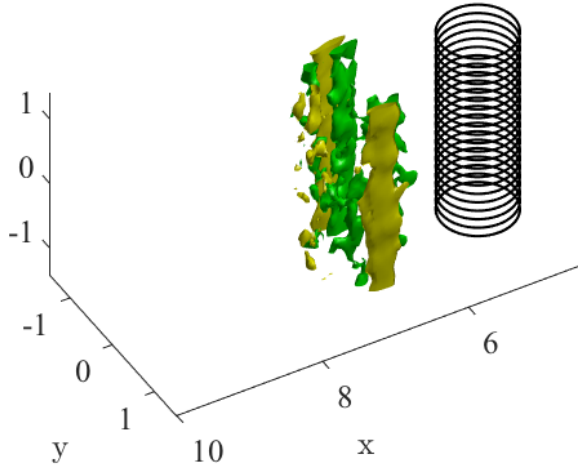
(e) \frac{1}{2}|\nabla \times (\nabla \cdot \mathbf{z}_2)^T| = 0.08
