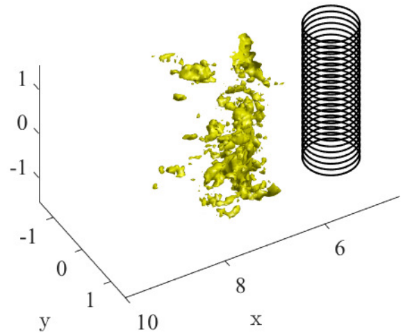
(e) \sqrt{\lambda_4}tr(\mathbf{z}_4) = 0.007
