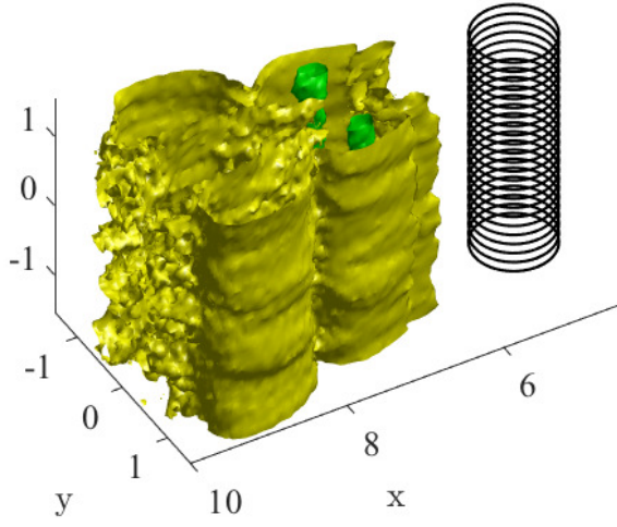
(b) \sqrt{\lambda_1}tr(\mathbf{z}_1) = (0.03; 0.007)
