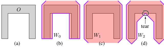
Figure 5: (a) O is an upside-down cubical mug without handle. The volumes W_i are illustrated in transparent red color. (b) We have W_0 = \text{PROPAGATEUP}(O') where the slices of O' are dilations of those of O . (c) W_1 = \text{PROPAGATEDOWN}(W_0) . (d) W_2 = \text{TIGHTDOWNWARDPROPAGATION}(W_0) .
