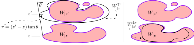
Figure 3: View of slices of W at height z (bottom) and z' (top). Left. The large component of W_{|z'} is included in W_{|z}^{\uparrow r} but its small component is not. Right. The small component has disappeared from W_{|z'}^{\downarrow r} so that W_{|z'}^{\downarrow r} \subset W_{|z} .
