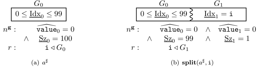
Figure 8: Partition splitting in array a from abstract state a^\#
