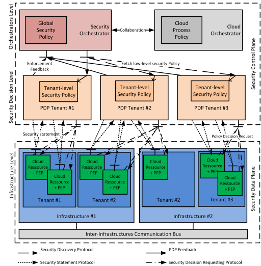
Figure 1. Proposed architecture for SDCSec in distributed cloud
