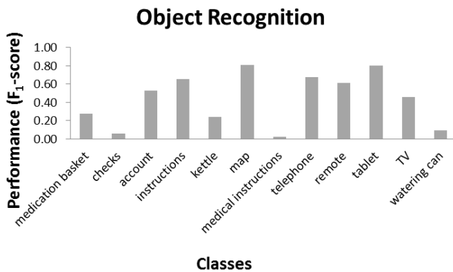
Fig. 8. Performance of OR concept detector per object class
