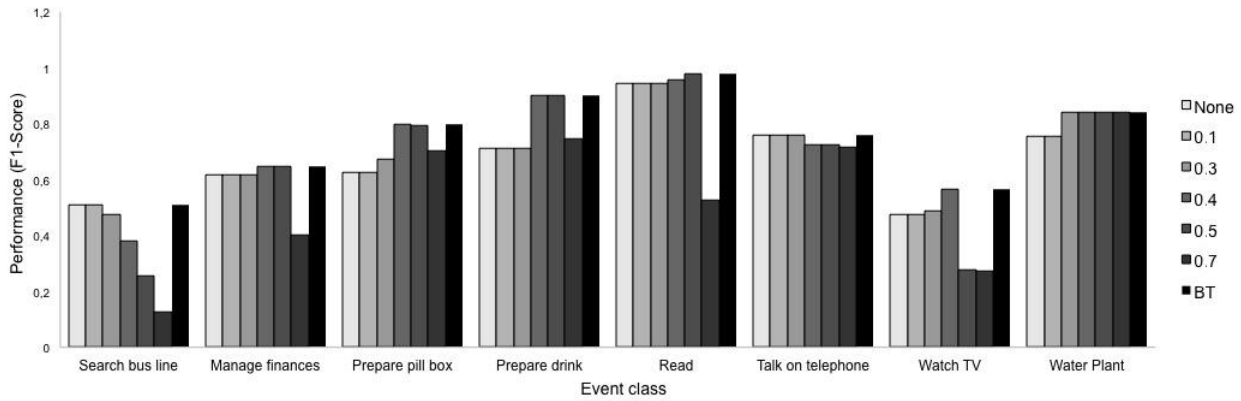
Event recognition performance versus probability threshold
