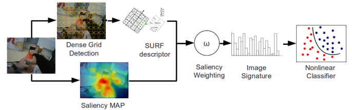
Fig. 2. Processing pipeline for saliency-based object recognition in first-person camera videos
