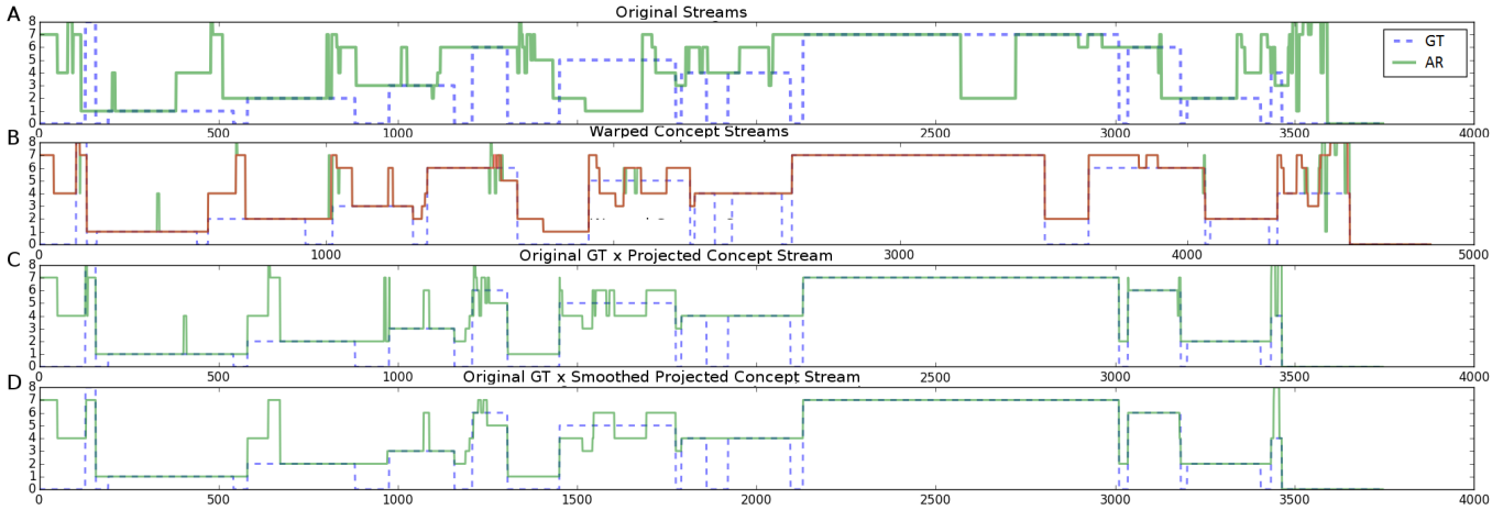
Fig. 6. Semantic alignment between the concept stream of the action recognition detector (AR) and a concept stream (GT) generated from events manually annotated by domain experts using the time axis of the color-depth camera. X-axis denotes time in frames, and Y-axis denotes activity code (1-8), respectively, search bus line on the map, establish bank account balance, prepare pill box, prepare a drink, read, talk on the telephone, watch tv, and water the plant. From top to bottom, images denote: (A) original GT and AR streams, (B) GT and AR streams warped, AR stream warped and smoothed (in red), (C) original GT and AR stream warped and then backprojected onto GT temporal axis, (D) original GT and AR warped, backprojected, and then smoothed with median filtering.
