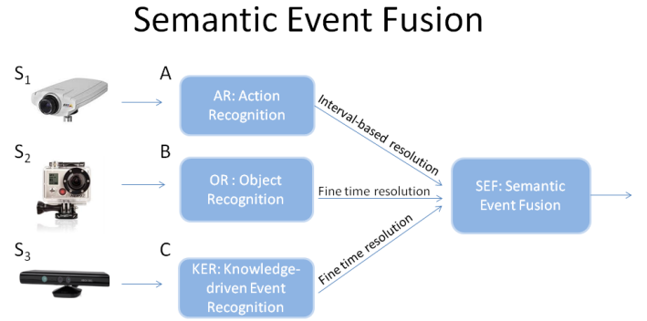
Fig. 1. Semantic event fusion framework: detector modules (A-C) process data from their respective sensors ( S_1 - S_3 ) and output concepts (objects and low-level events). Semantic Event Fusion uses the ontological representation to initialize concepts to event models and then infer complex, composite activities. Concept fusion is performed on millisecond temporal resolution to cope with instantaneous errors of concept recognition.
