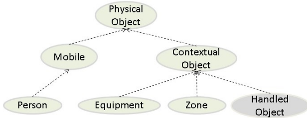
Fig. 3. Physical object sub-tree of the ontology language
