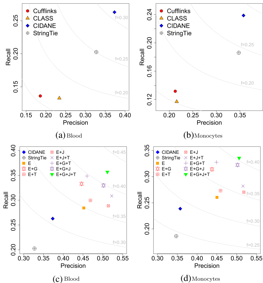
Fig. 5 Recall and precision on real human data. a, b Ab initio transcript predictions. Isolasso and MITIE with recall values of 5–8 % are omitted (see Additional file 1: Table S7). c, d Recall and precision of annotation-guided assemblies by CIDANE. Ab initio predictions of CIDANE and StringTie shown as reference. In addition to read alignments, CIDANE employs information on exon boundary (E), gene boundary (G), TSS/TES (T), and exon junction (J). Same color of symbols indicates same number of augmentary information types
