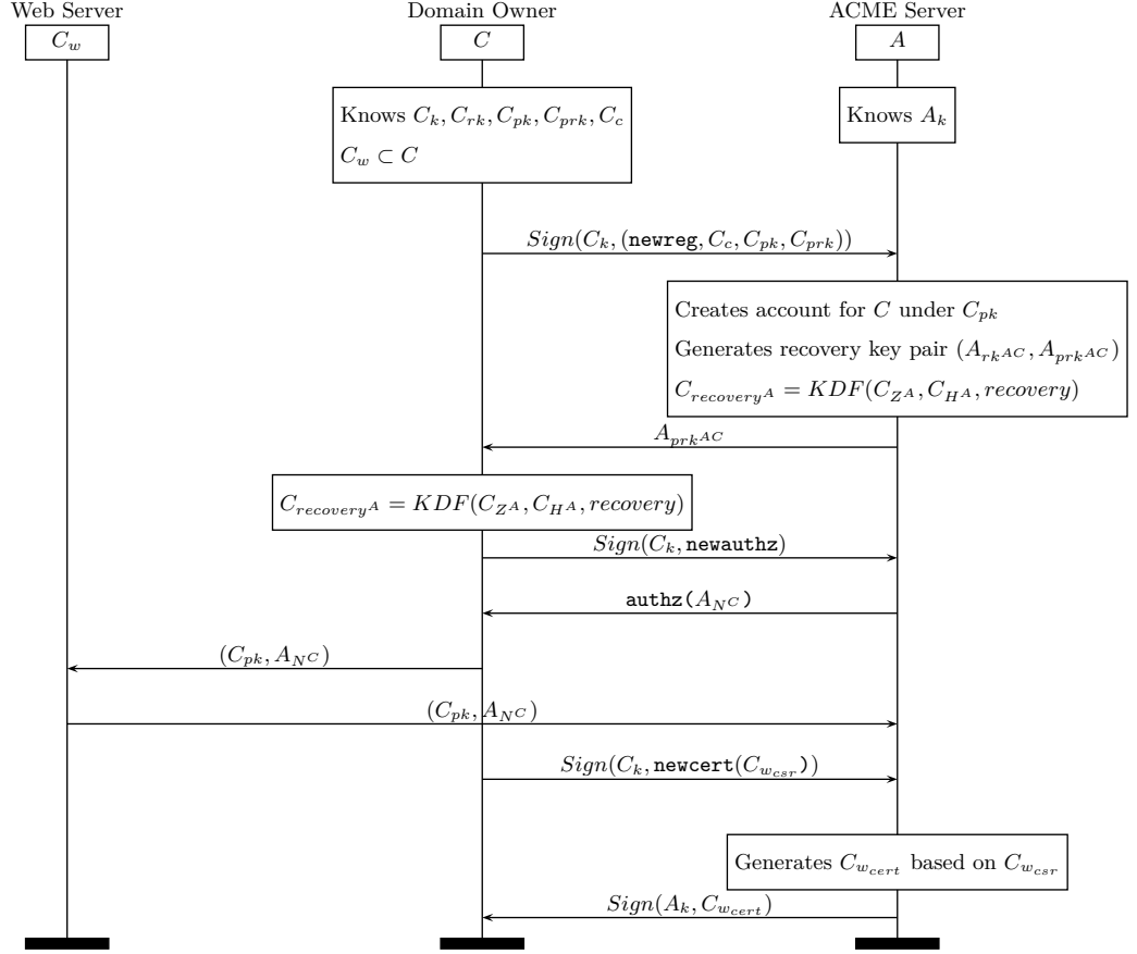
Fig. 4: ACME draft-1 protocol functionality for C account registration, recovery key generation, and validation with certificate issuance for C_w . This chart demonstrates validation via an HTTP identifier. In draft-3 and above, the HTTP challenge (C_{pk}, A_{NC}) is replaced with \text{Sign}(C_k, (C_{pk}, A_{NC})) .
