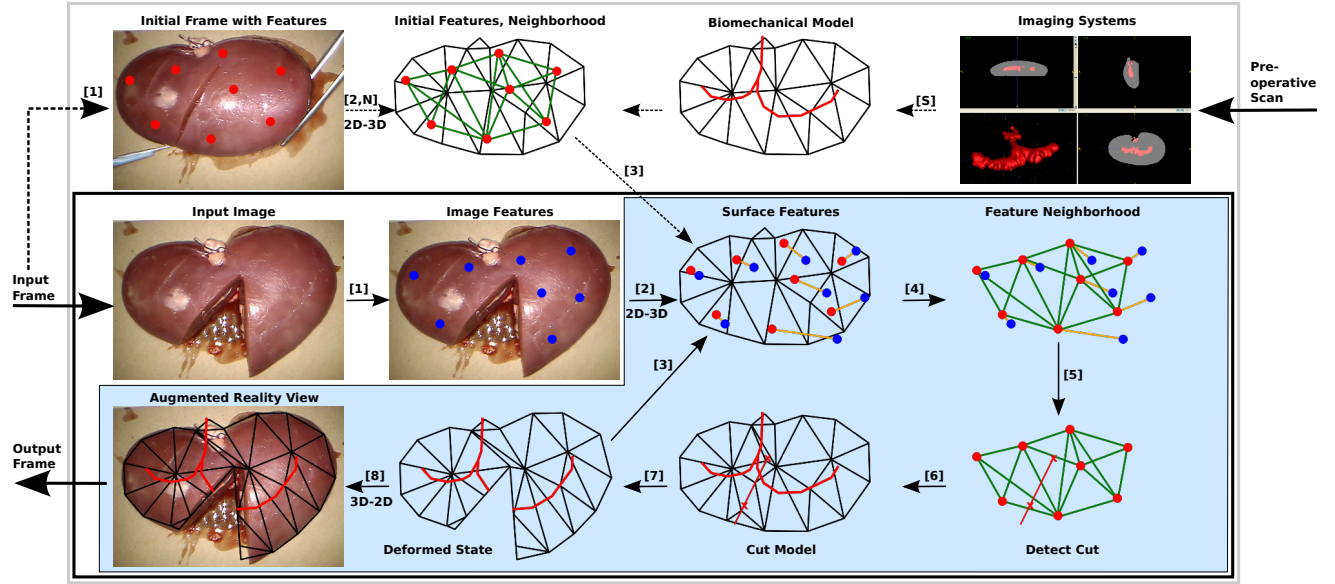
Fig. 1 Pipeline of our method: [S] Segmentation, [1] identify image features p_{l,f} (see 4.2), [2] map image features on model (see 4.2, 5.2), [N] construct feature neighbourhood C_F^0 (see 5.2), [3] use initial/updated model (P_V, C_V) and compare image p_{l,f} and surface features p_{l,F} by [4] calculating the measure \mu_{lm} on the neighborhood C_F^0 , [5] detect outliers, insert cut points p_C , expand cut points to cut lines, [6] expand cut line to cut surface S (see 5.2), update topology of model and internal structures (see 5.3, 5.4), [7] solve minimization problem (5) of 4.3, [8] display model on output frame; the dashed flashes are performed at initialization; one frame with image features can be used several times, repeating the steps [2]-[8] in the blue area.
