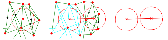
Fig. 2 From left to right: insertion of a cut point based on the barycenters of identified outliers (black crosses); update of the connectivity information (turquoise connections are not used any more), insertion of a second cut point yields a cut line (polygon); cut polygon is extended until the end of its radius r_{p_C}
