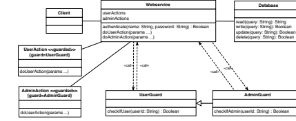
Fig. 4. Secure Guards in UMLsec
