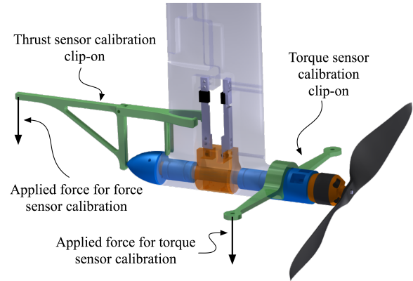
Fig. 7: Clip-on calibration parts.
