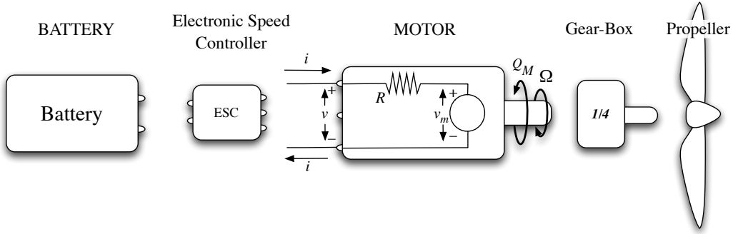
Fig. 1: Elements of a generic electric propulsion system.
