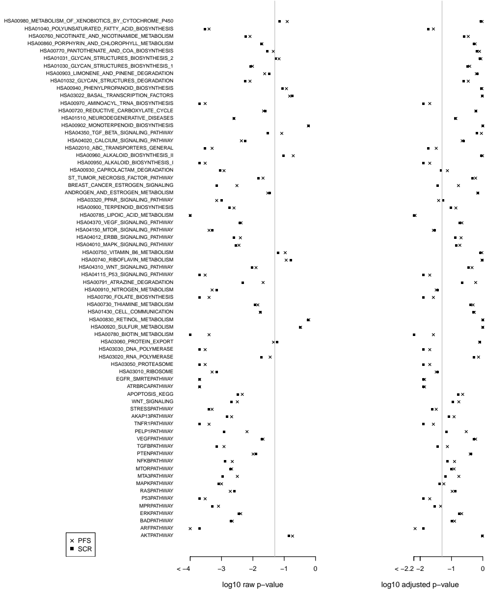
Figure 1. log10 p-values for testing the overall effect of 70 genetic pathways on breast cancer survival based on the KM (kernel machine) score test with Gaussian kernel using kernel PCA (principal components analysis; with a 90% of total variability threshold). The crosses and the squares represent PFS and SCR models, respectively. These results are based on B = 20,000 perturbations.
