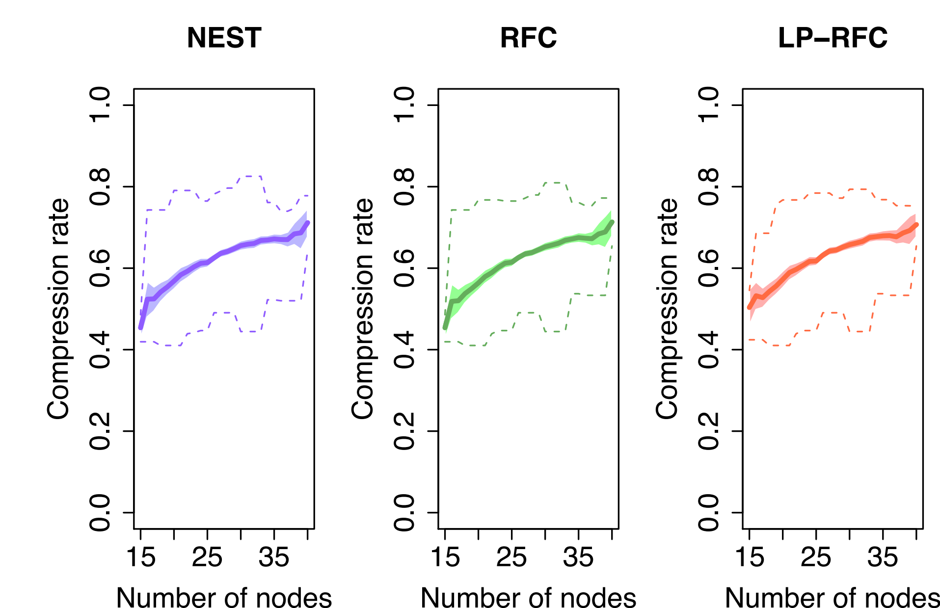
Figure 3: Compression rates on the simulated dataset.
