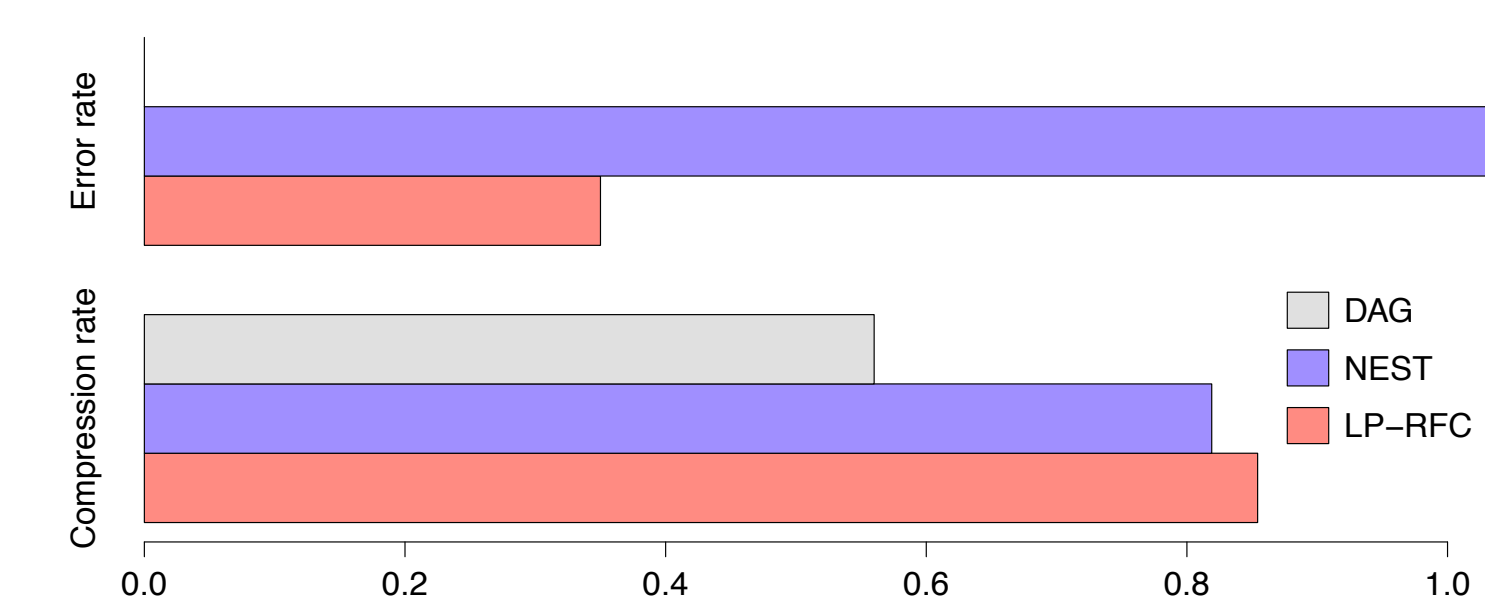
Figure 1: Error and compression rates on the example.
