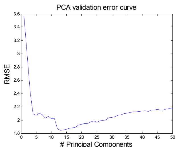
Fig. 5: PCA-ELM validation error curve for Connecticut Site
