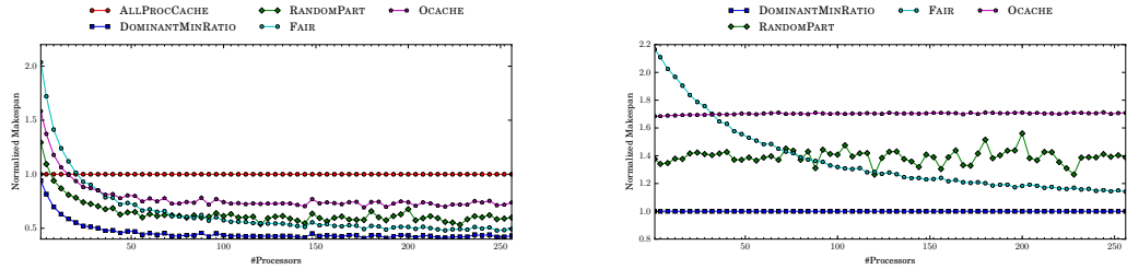
Figure 10: Impact of the number of processors with NPB-6.
