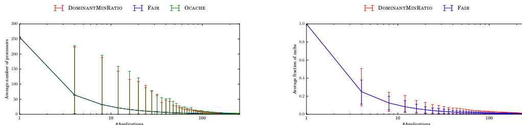
Figure 17: Processor and cache repartition with 256 processors with RANDOM.
