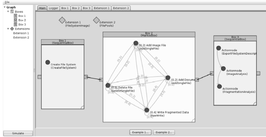
Figure 3. Screenshot of the model builder.
